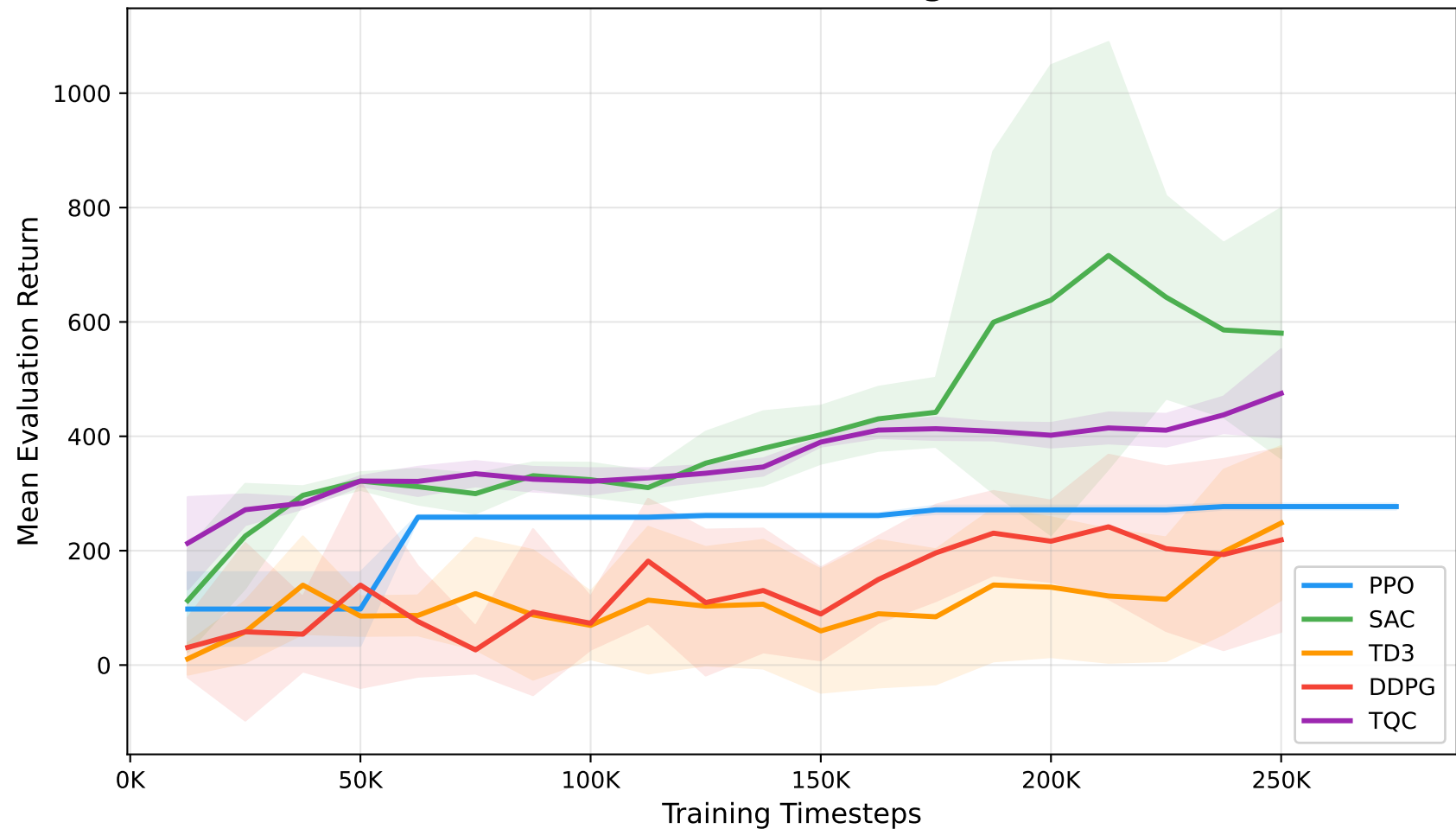
Walker2d-v5 — Learning Curves
