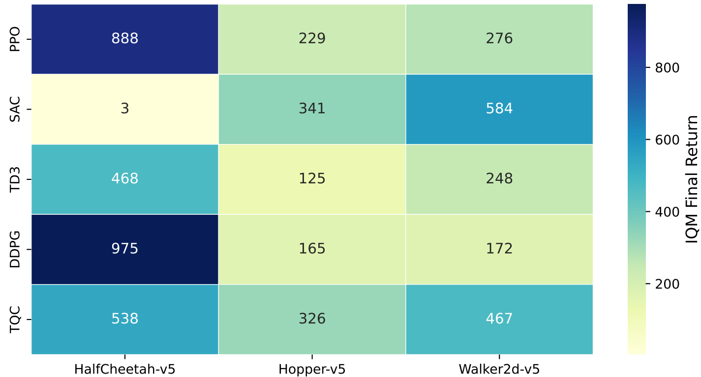
Algorithm × Environment Performance (IQM)
