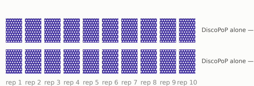
no_evidence_nospeed_v4 · claude-haiku-4-5-20251001
