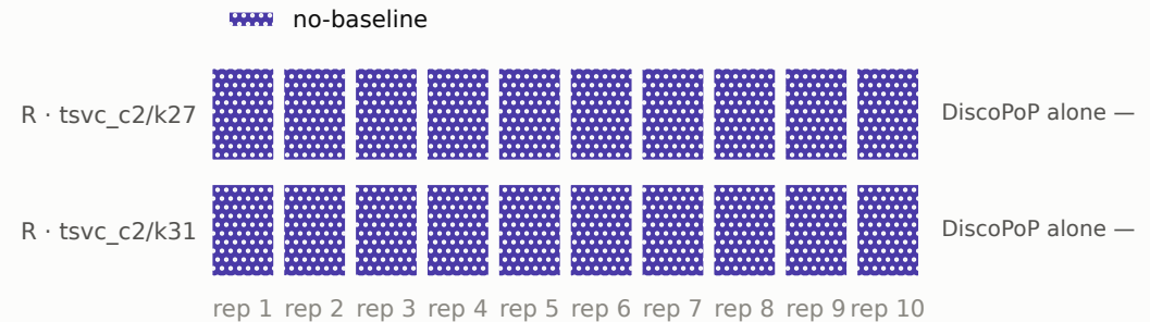
full_nospeed_v4 · claude-haiku-4-5-20251001
