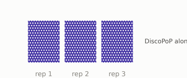
llm_pragmas_v5 · claude-haiku-4-5-20251001
