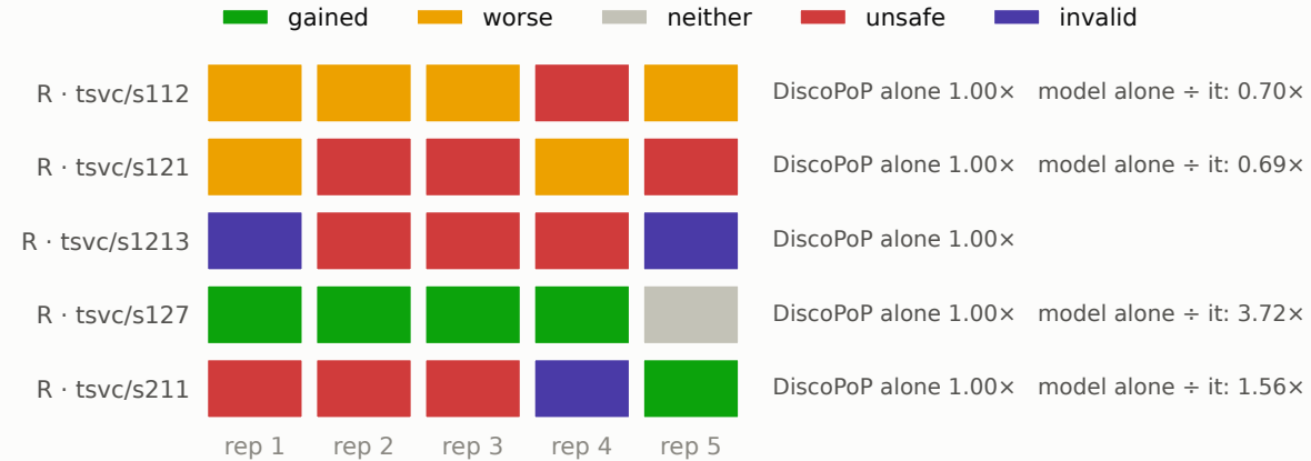
bare_llm · claude-haiku-4-5-20251001
