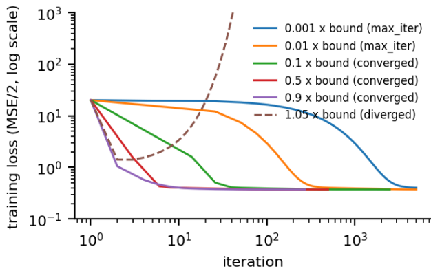
Figure 1a. Phase 1 loss for six learning rates given as fractions of the stability bound: stall, converge, diverge.
