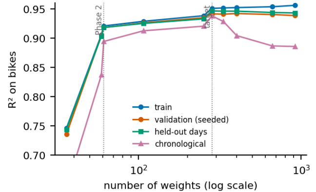
Figure 1b. Phase 3 ladder: training R^2 keeps rising with the number of weights; the three held-out estimates peak at the target and then fall, the chronological one most.
