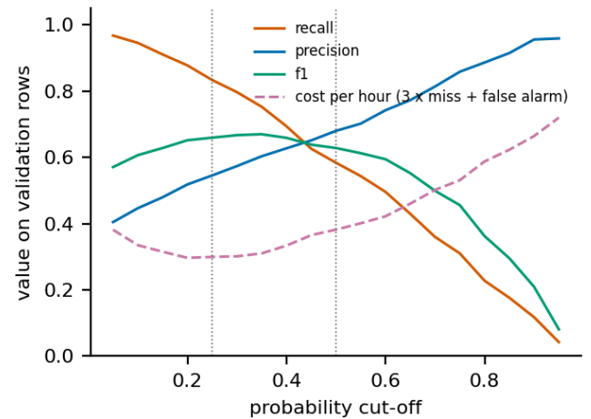
Figure 2b. Phase 5: precision, recall, F1 and operator cost against the probability cut-off (dotted lines: 0.25 and 0.5).
