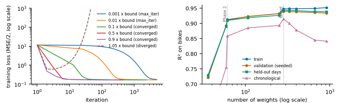
Figure 1a. Phase 1 loss for six learning rates given as fractions of the stability bound: stall, converge, diverge. Figure 1b. Phase 3 ladder: training R^2 keeps rising with the number of weights; the three held-out estimates peak at the target and then fall,
