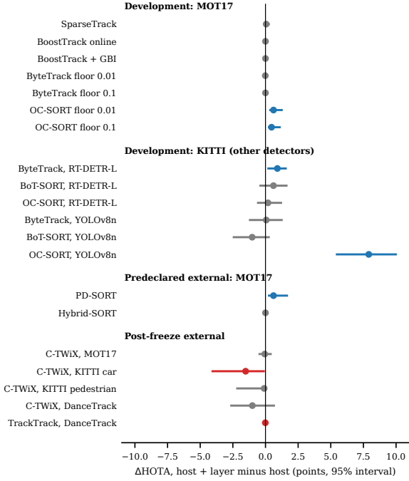
Fig. 3 Difference in HOTA (host with SCL minus host alone) with 95% paired-bootstrap interval for every evaluated cell. Blue: above zero; red: below zero; gray: includes zero or identical output.
