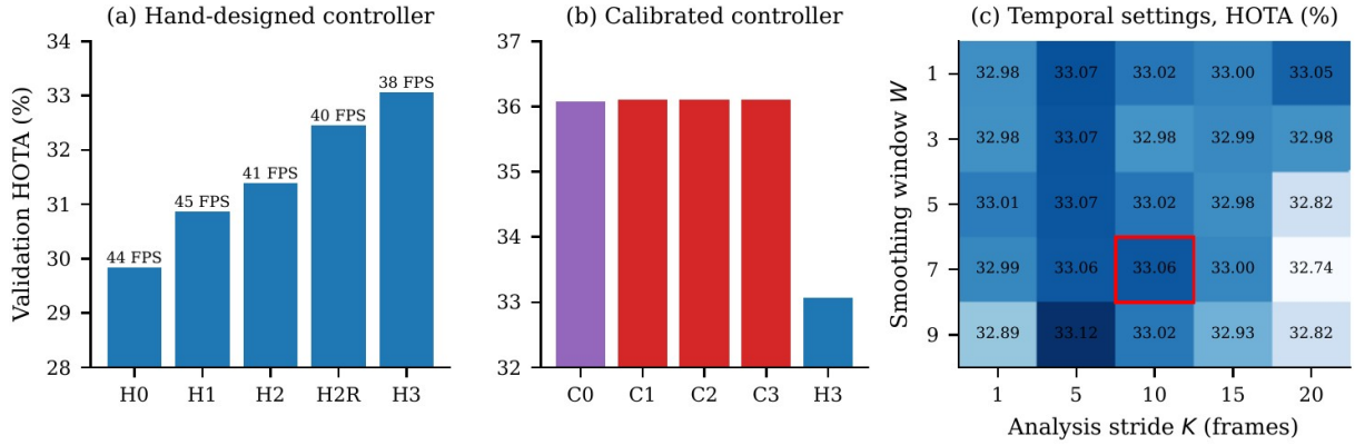
Fig. (4.5) Validation ablations.
