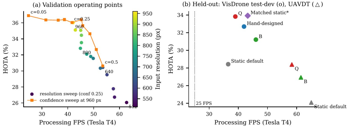
Fig. (4.6) Accuracy versus processing throughput on one Tesla T4.
