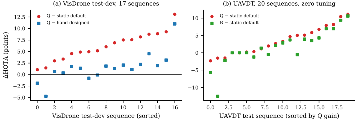
Fig. (4.4) Per-sequence HOTA differences, sorted.
