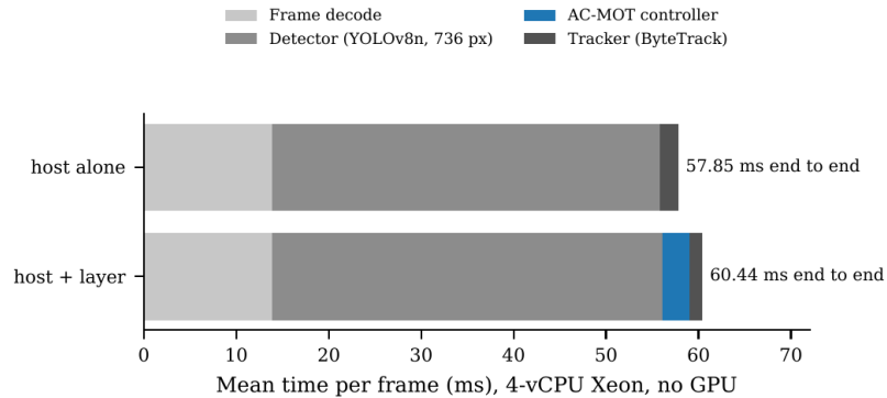
Fig. (5.7) Mean per-frame time by stage without and with the layer.
