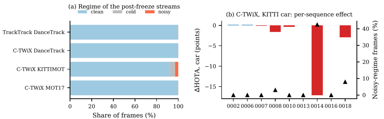
Fig. (5.6) (a) Share of frames in each regime on the post-freeze streams.
