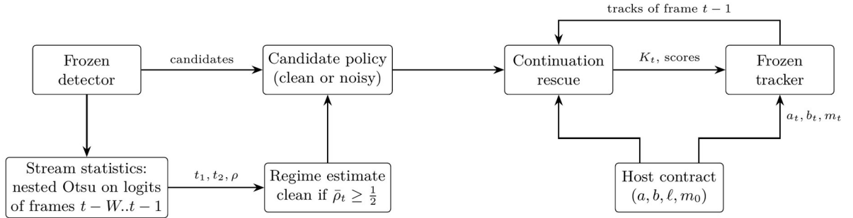
Fig. (5.1) Self-calibrating control layer between a frozen detector and a frozen tracker.
