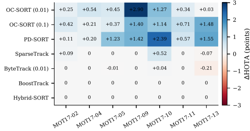
Fig. (5.4) Per-sequence HOTA differences on MOT17 val-half for development and predeclared trackers.
