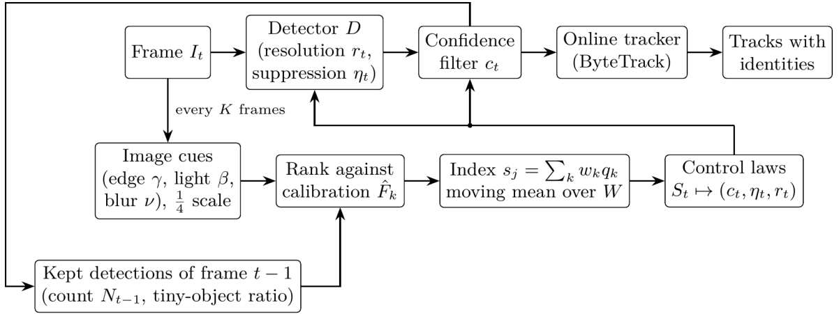
Fig. (4.1) Scene-adaptive operating-point control.
