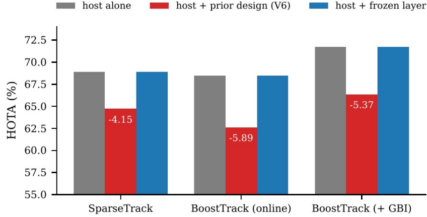
Fig. (5.2) The design problem: the prior always-intervening design degraded strong published trackers on MOT17 (difference in white); the frozen layer leaves them at their own accuracy.
