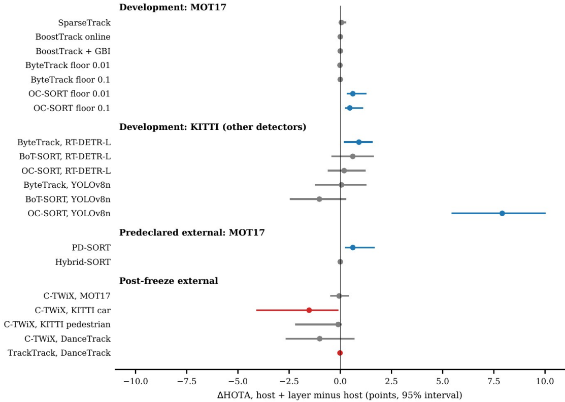
Fig. (5.3) Every evaluated cell: difference in HOTA (tracker with the frozen layer minus tracker alone) with 95% paired-bootstrap interval.
