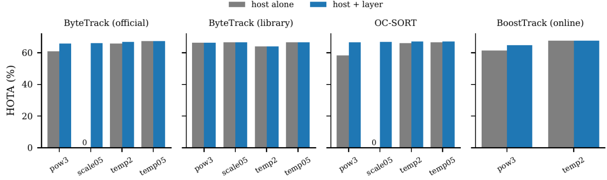
Fig. (5.5) Detector confidence shift on MOT17 val-half: HOTA of each published tracker with its published thresholds, alone and with the frozen layer, after four monotone transforms of the detector scores.
