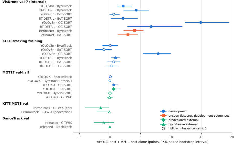
Fig. 5 HOTA difference (host with the frozen layer minus host alone) with 95% paired bootstrap intervals for every recorded combination, grouped by dataset and marked by evidence status. Filled markers: interval excludes zero. VisDrone rows use the frozen General AC-MOT configuration (V7f at 736 px); KITTI values are KITTI HOTA (car/pedestrian mean).
