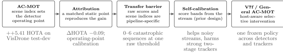
Fig. 1 From AC-MOT to General AC-MOT. The scene-adaptive controller worked; attribution showed that its gain came from a calibrated operating point; transferring that calibration through raw scores or scene indices failed across detectors and pipelines; self-calibrated score bands fixed noisy detector streams but harmed well-matched trackers; the final layer self-calibrates and intervenes only when the tracker’s declared operating point does not fit the stream.
