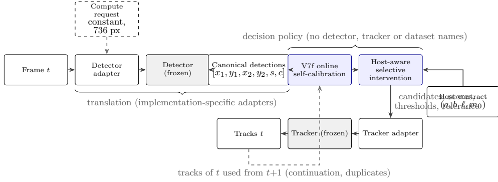
Fig. 2 Architecture of General AC-MOT. Adapters translate model-specific interfaces; the V7f policy decides from the score stream of previous frames, the tracker’s declared host contract and the tracks of the previous frame. Detector and tracker are frozen. The compute request is constant in the frozen system.
