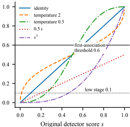
(a) Score recalibrations used in the stress test
