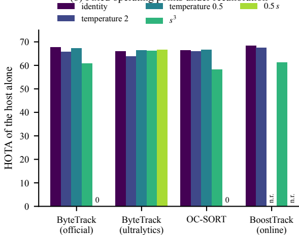
(b) Fixed operating points under recalibration
