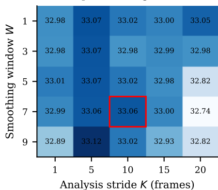
(c) Temporal settings, HOTA (%)
