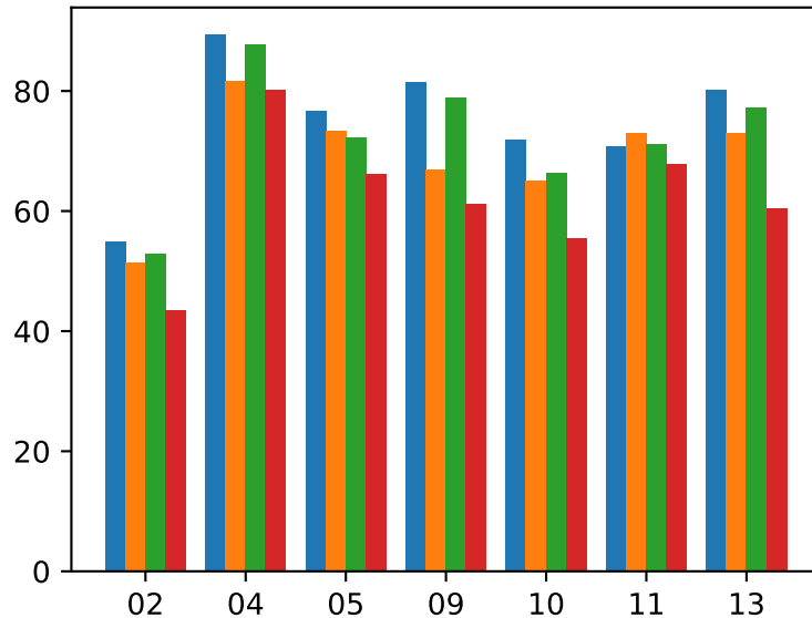
MOT17 val-half per-sequence MOTA
