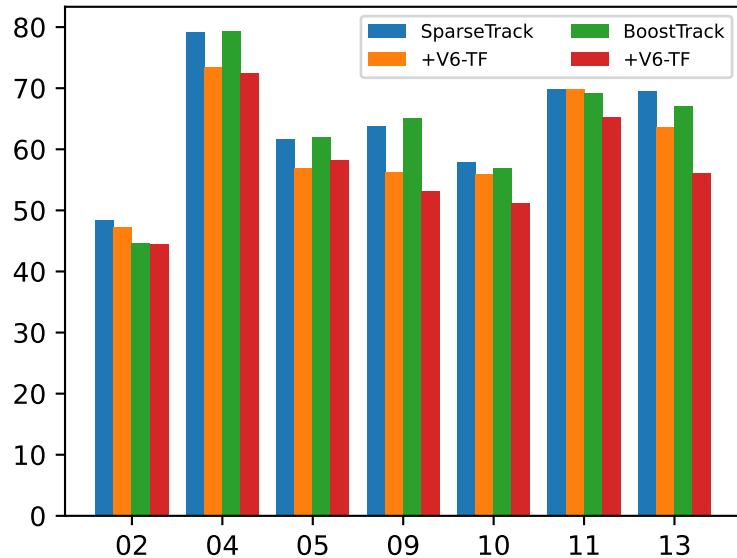
MOT17 val-half per-sequence HOTA
