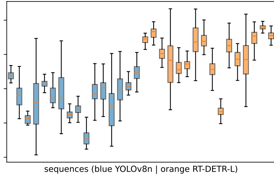
conf16: per-sequence primary threshold
