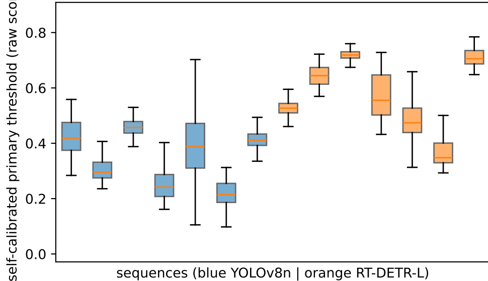
val7: per-sequence primary threshold
