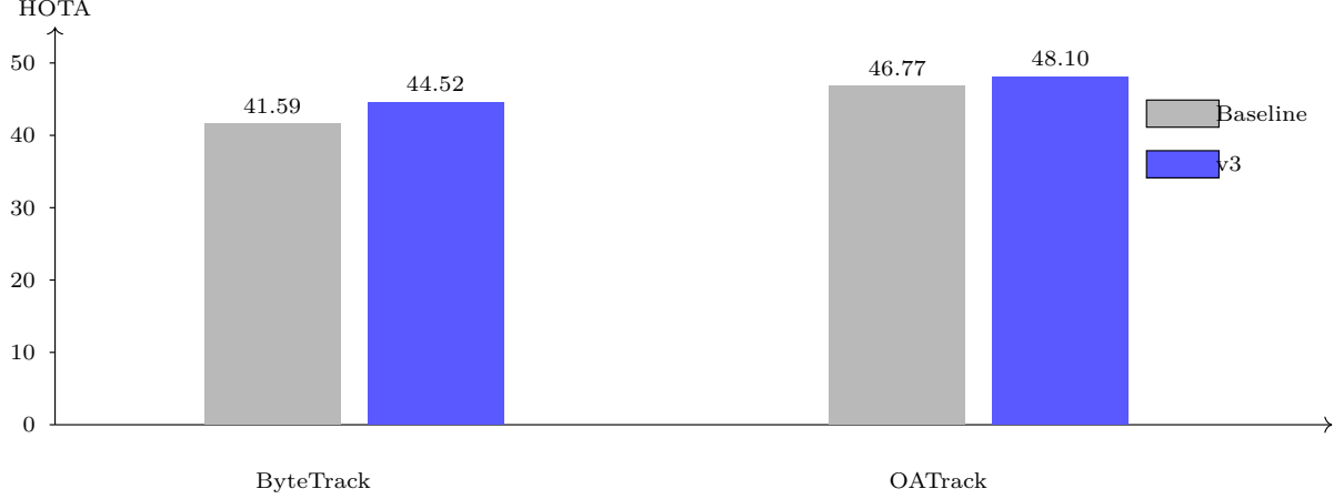
Fig. 4 Modern VisDrone second-read results on seven sequences; hosts are evaluated separately under the custom protocol.
