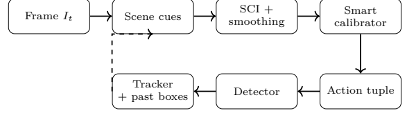
Fig. 2 Original causal AC-MOT flow; prior tracker boxes feed the next analysis.
