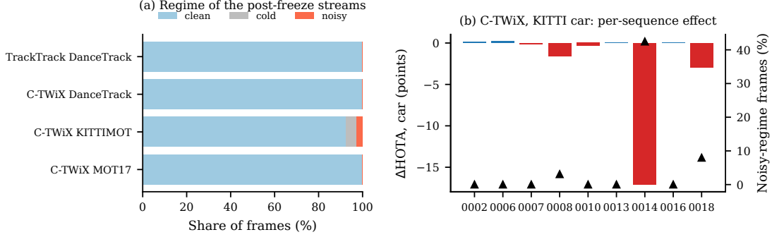
Fig. 4 (a) Share of frames in each regime on the post-freeze streams. (b) C-TWiX on KITTI cars: per-sequence HOTA difference (bars) and share of frames classified noisy (triangles).
