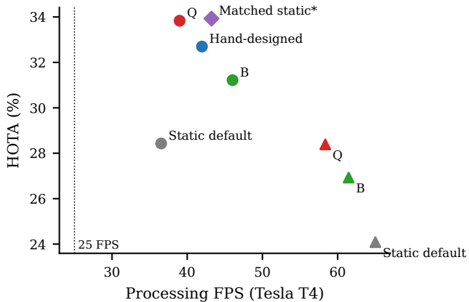
(b) Held-out: VisDrone test-dev (o), UAVDT ( \Delta )
