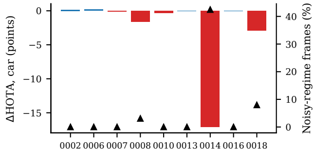
(b) C-TWiX, KITTI car: per-sequence effect
