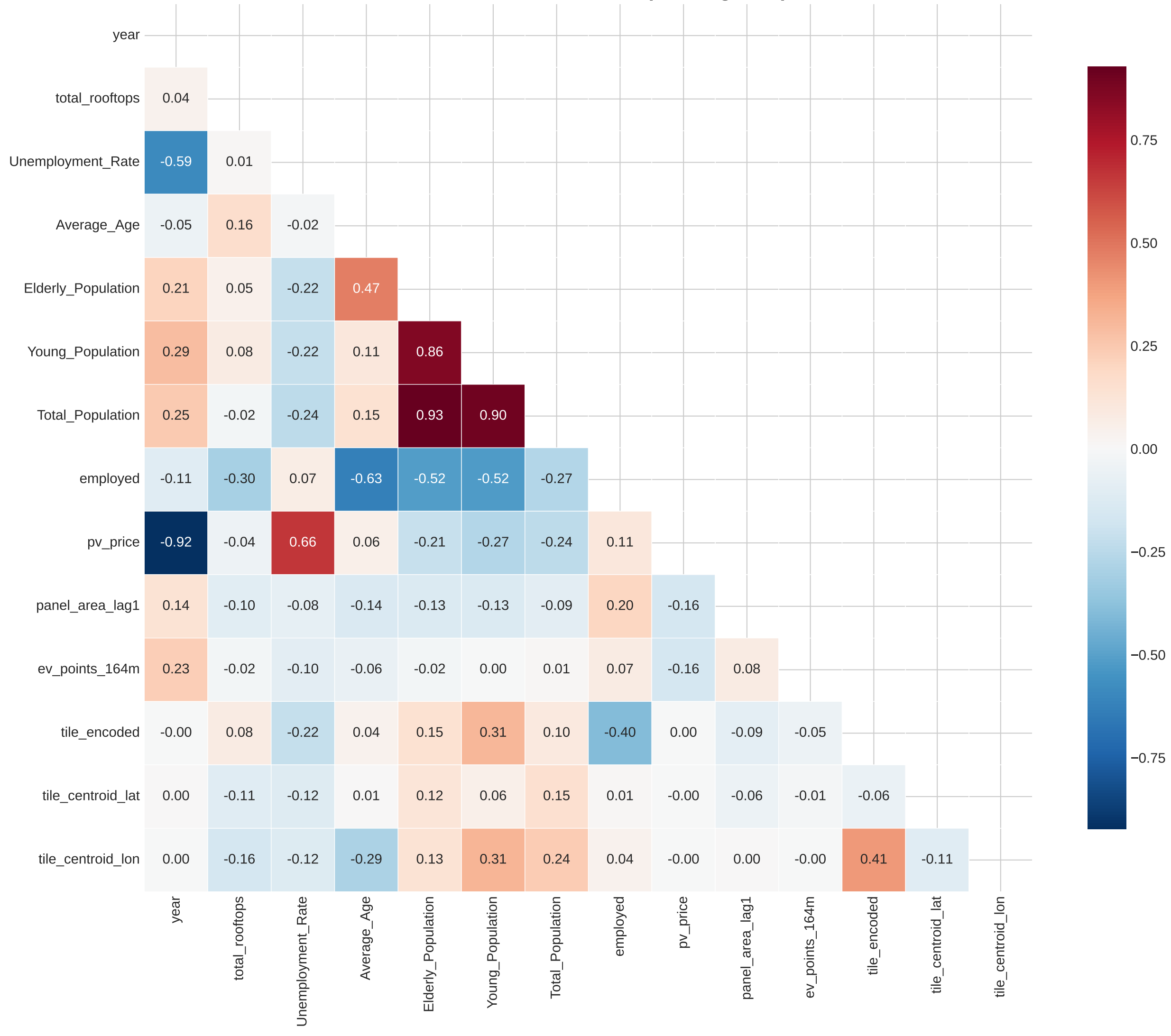
Feature Correlation Matrix (Training Data)
