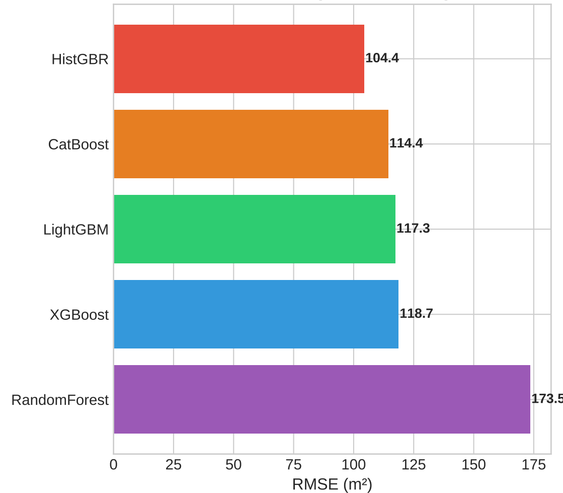
Test RMSE (lower = better)
