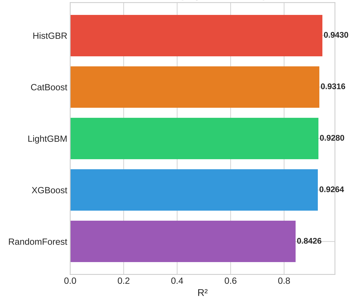
Test R² (higher = better)
