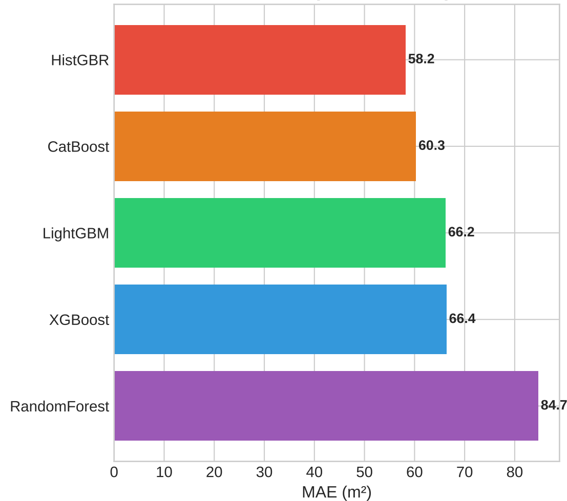
Test MAE (lower = better)
