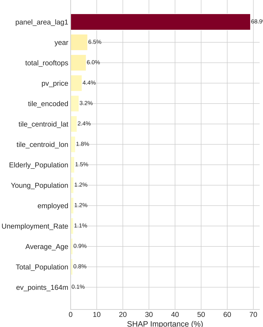
LightGBM
