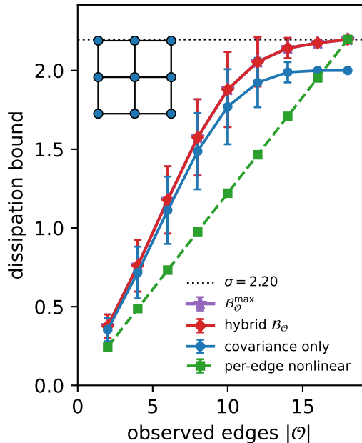
(a) 3 \times 3 torus, \gamma_G=0
