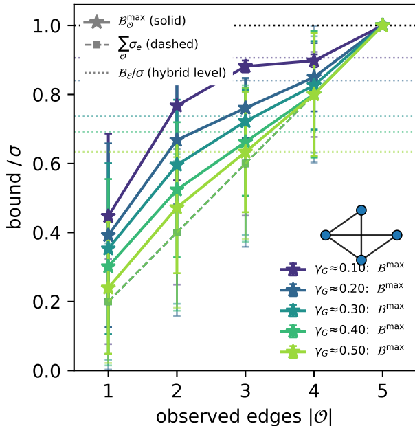
(b) 4-state two-cycle, \gamma_G sweep
