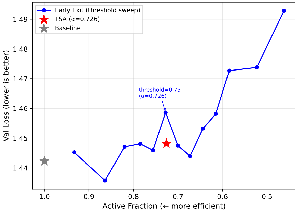
Early Exit vs TSA — Quality-Efficiency Pareto
