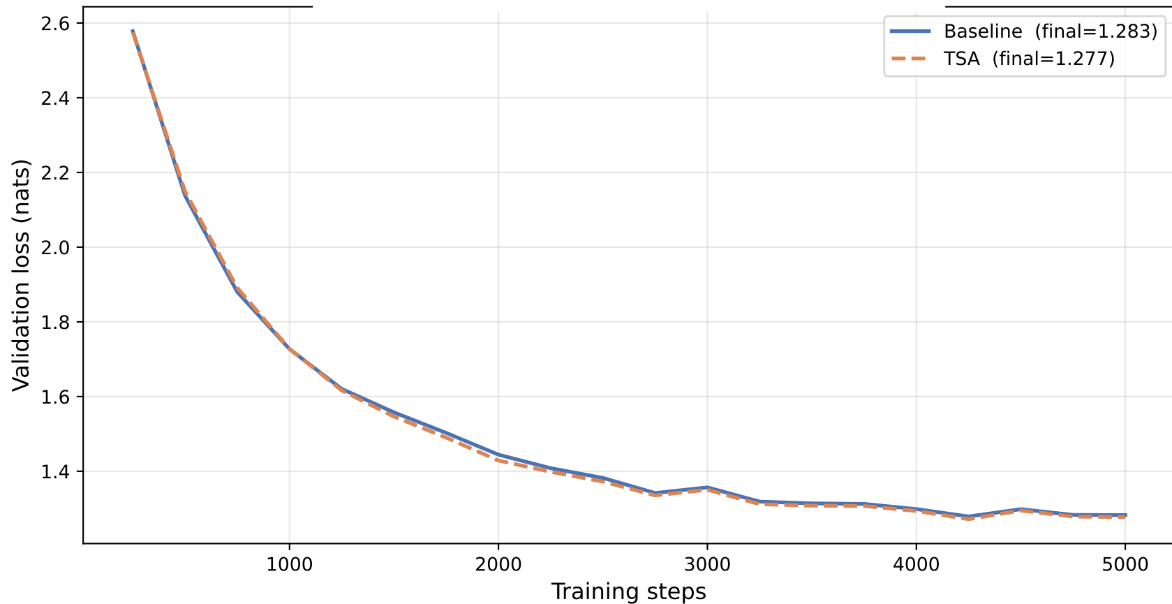
enwik8: Validation Loss vs. Training Step
