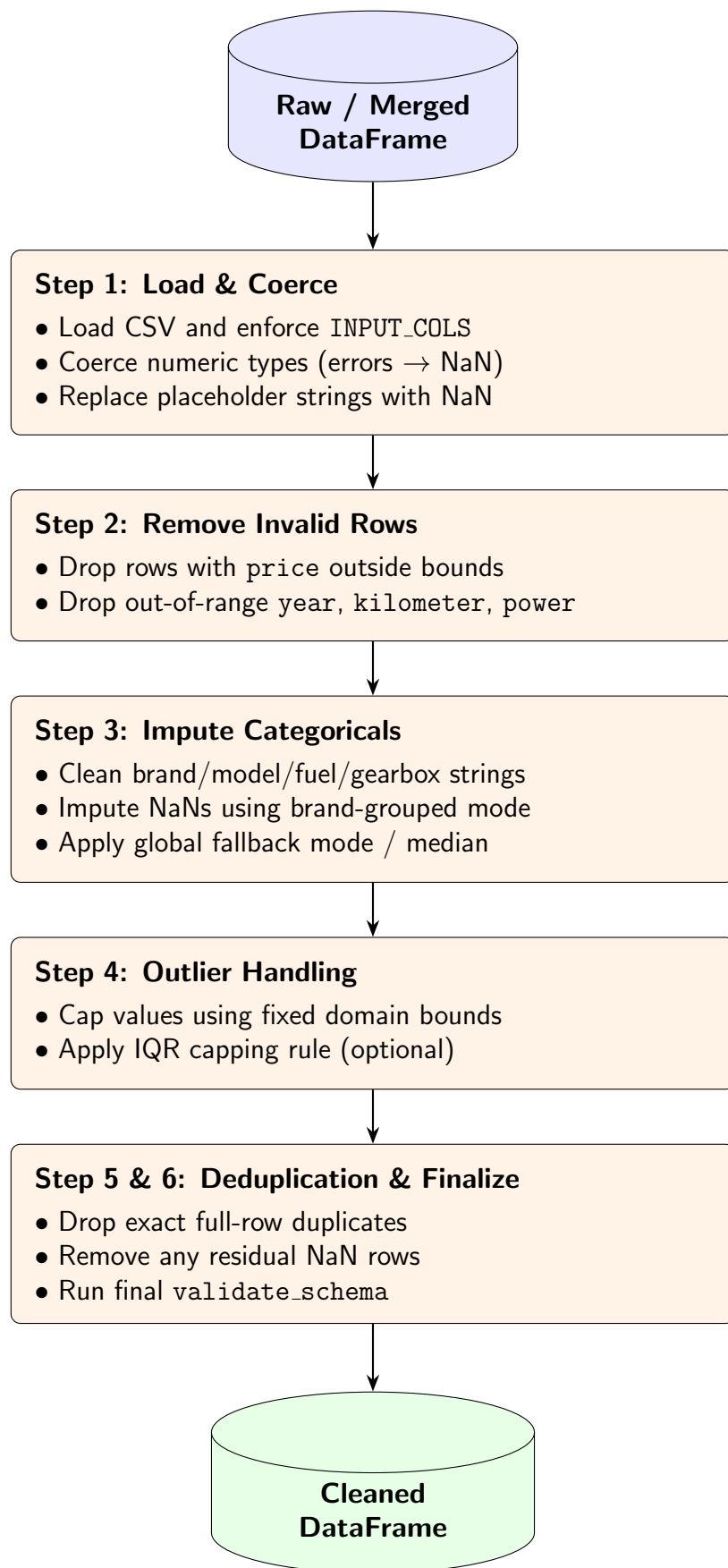
Figure 3: Data Cleaning Pipeline Execution Flow
