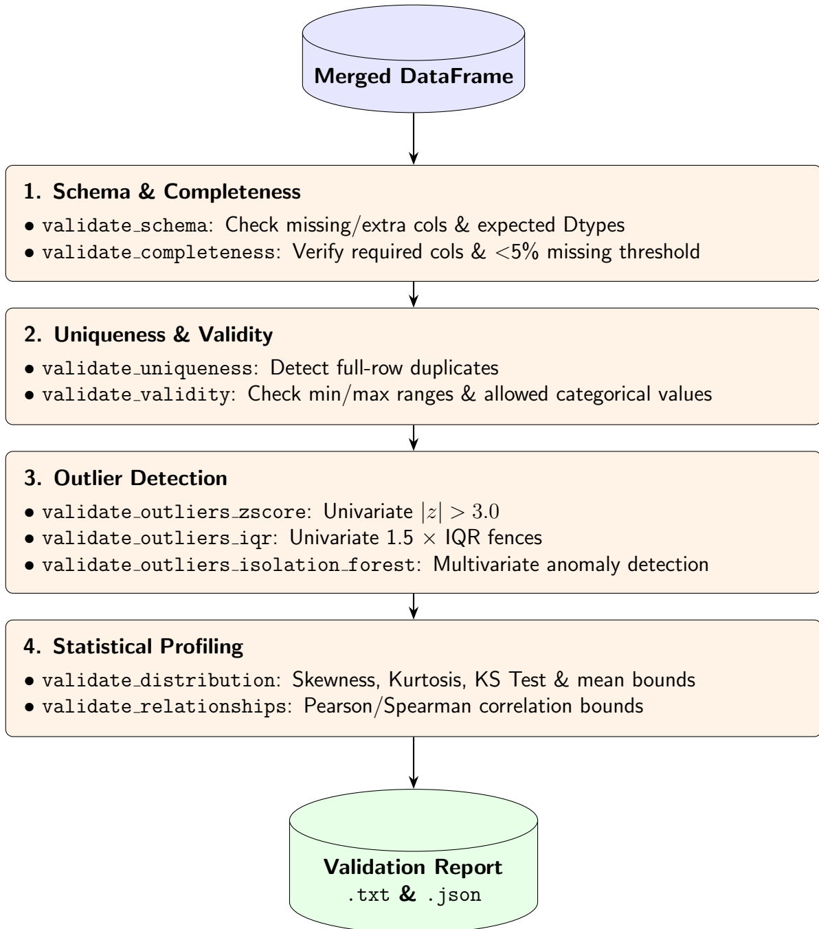
Figure 2: Data Validation Pipeline Execution Flow
