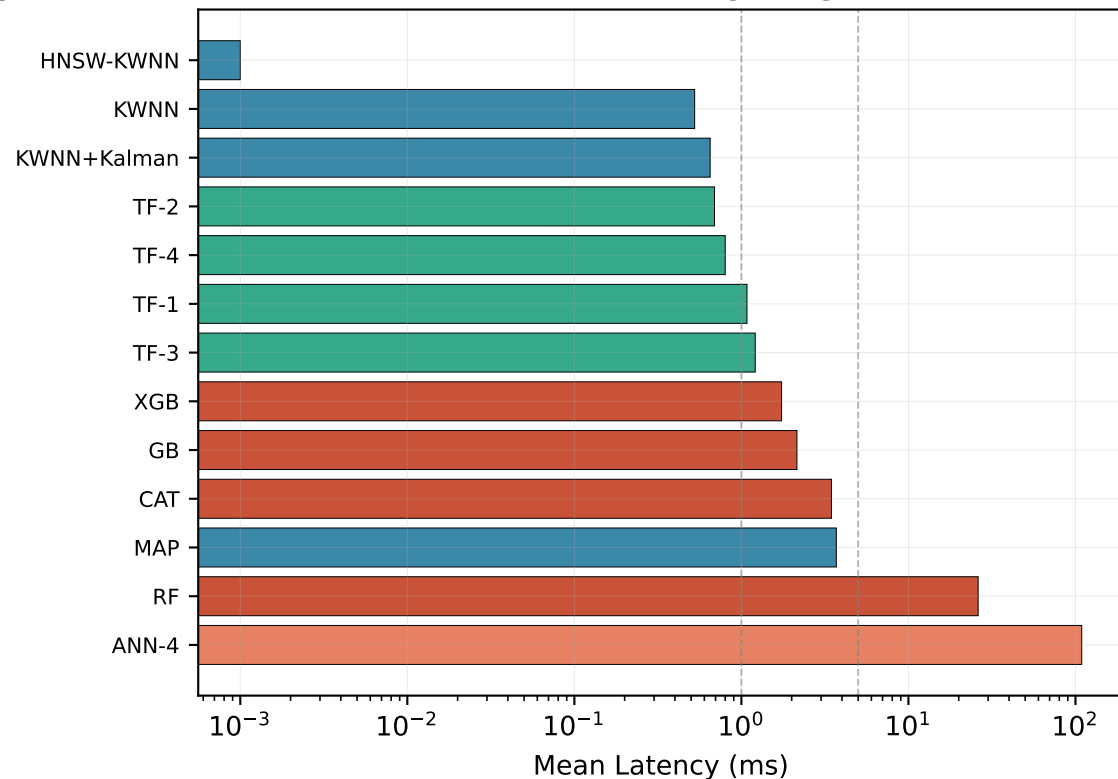
(b) Inference Latency (Log Scale)
