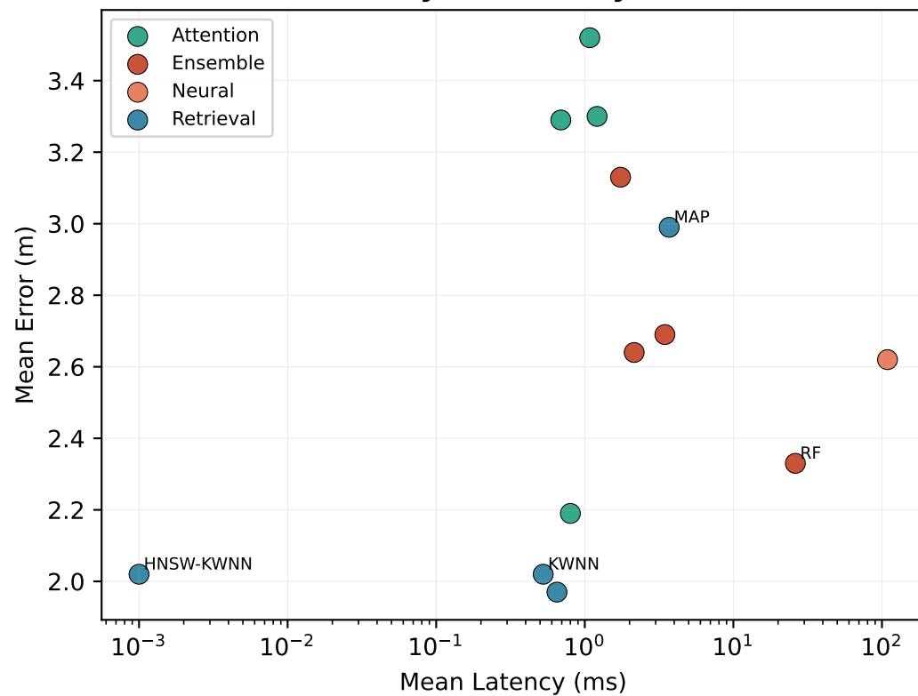
(c) Accuracy vs. Latency Trade-off
