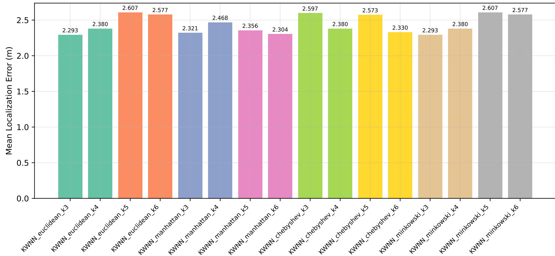
KWNN: All Distance Metrics x k Values
