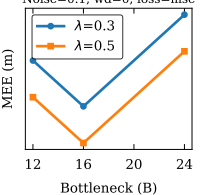
Noise=0.1, wd=0, loss=mse
