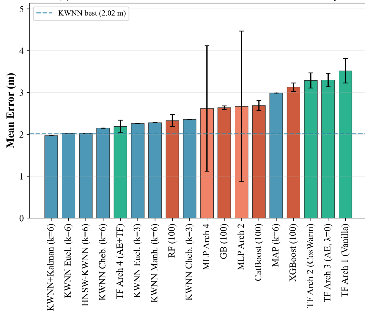
(a) Mean Localization Error with Cross-Seed Variability
