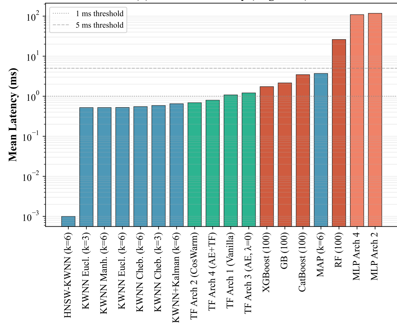
(b) Inference Latency (Log Scale)
