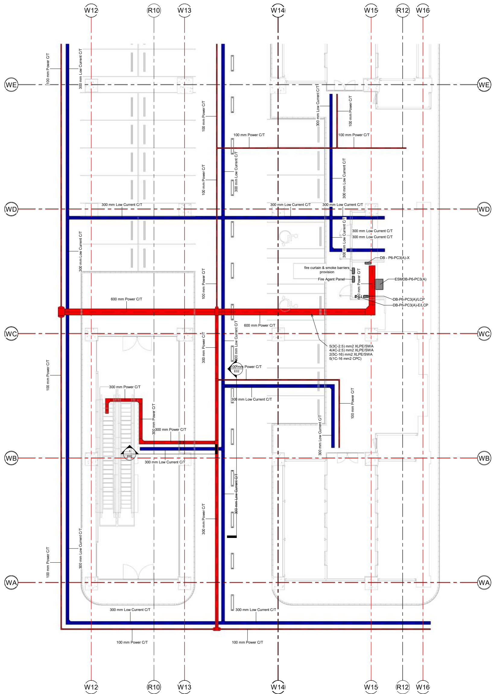
1 P06 - Cable Tray - WA/WE - W12/W16 1 : 100
