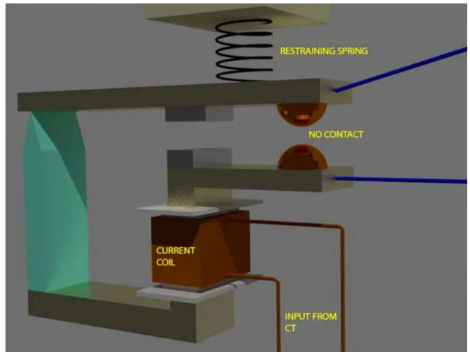
Figure 3: instantaneous over current relay components
