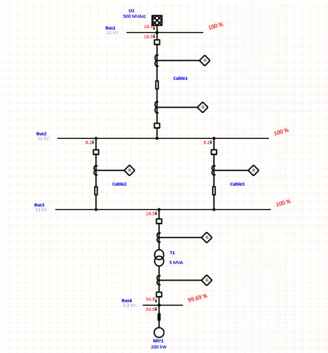
Figure 7: load flow of the system.
