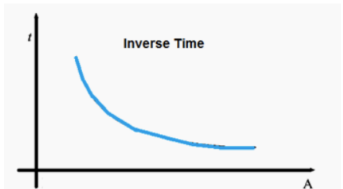
Figure 1: inverse over current relay curve
