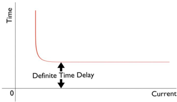
Figure 4: characteristics of definite time relay
