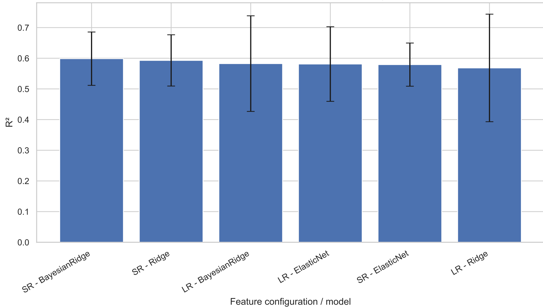
Top models: OOF R^2 and fold-to-fold variability
