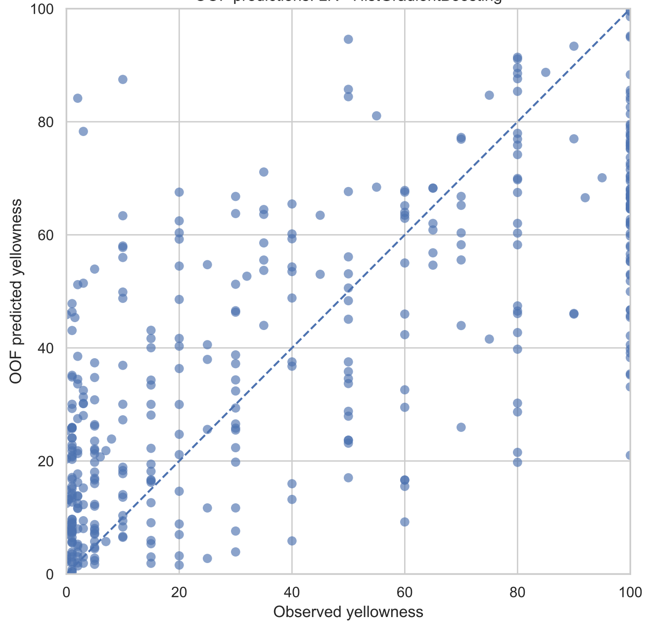
OOF predictions: LR - HistGradientBoosting
