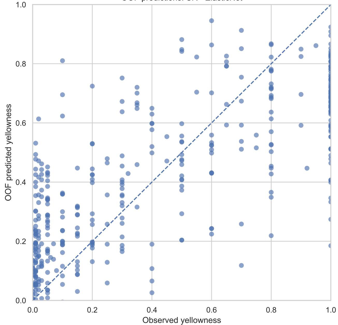
OOF predictions: SR - ElasticNet
