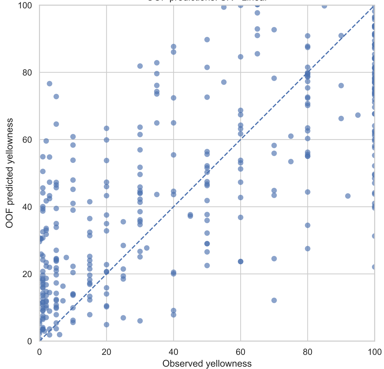
OOF predictions: SR - Linear
