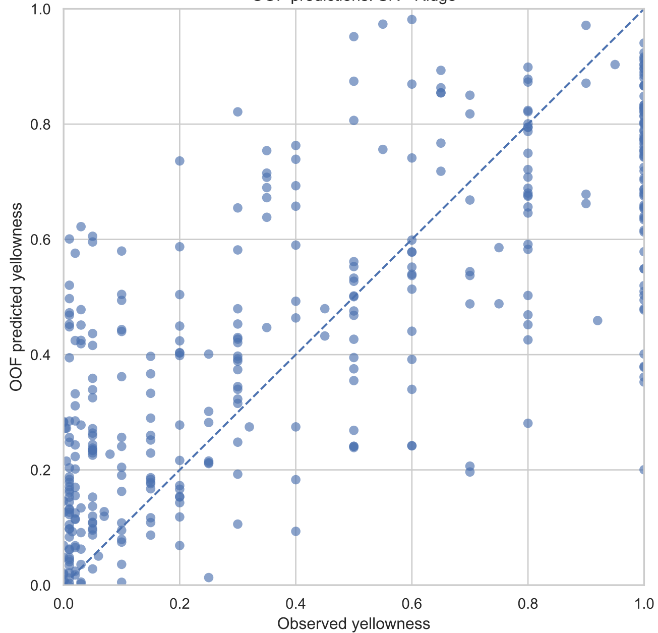
OOF predictions: SR - Ridge
