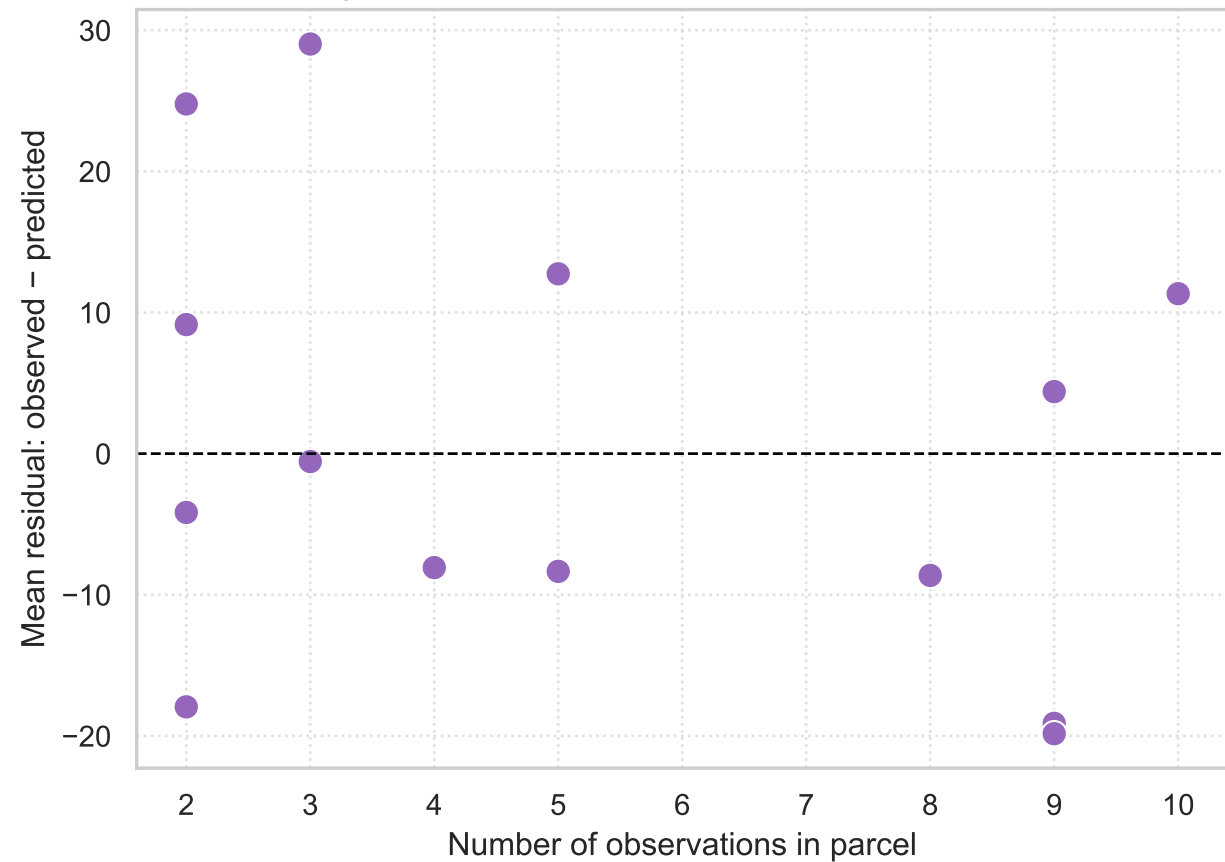
Deep Learning E4 validation: prediction bias versus number of observations
