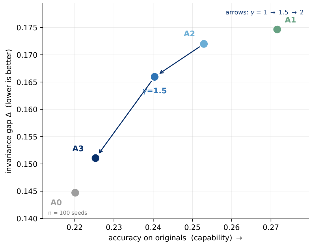
Capability vs invariance
