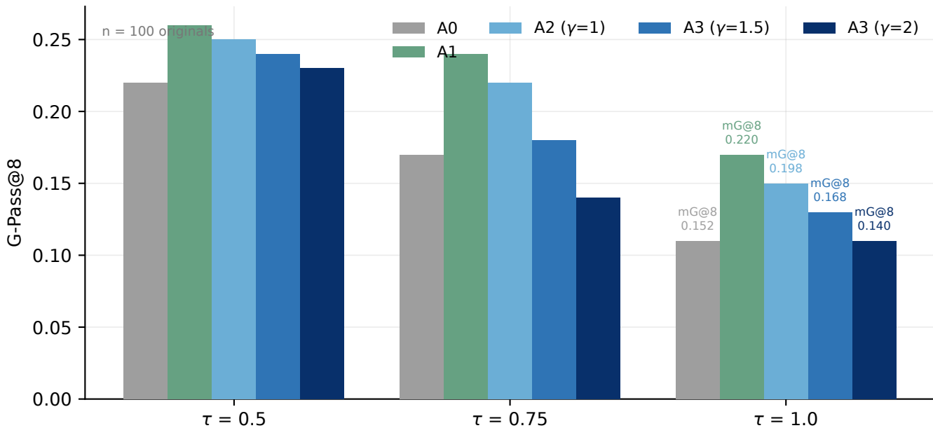
Reliability profile on ORIGINALS (variants were sampled once; G-Pass undefined there)
