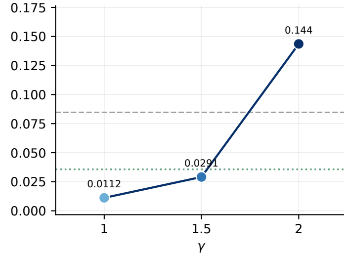
extract-fail rate (lower is better)
