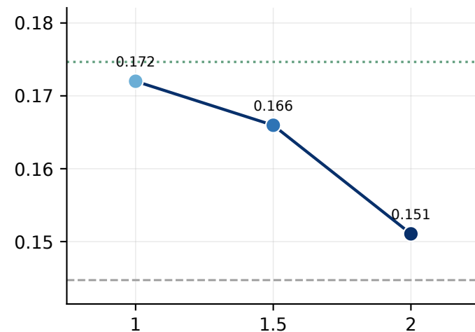
extract-fail rate (lower is better)
