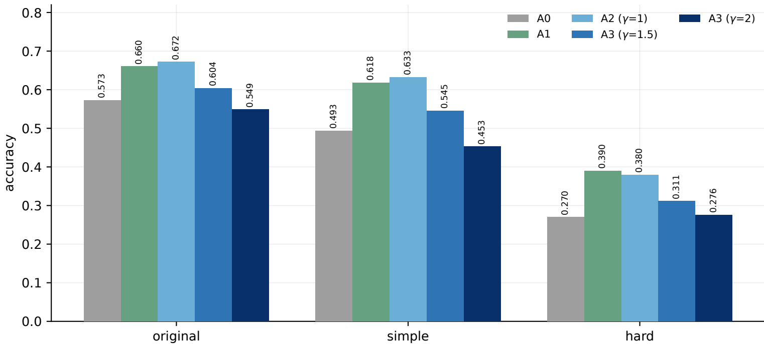
Accuracy by arm (n = 277 shared seeds)
