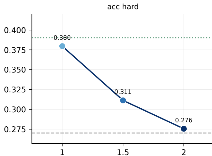
The \gamma path: \gamma = 1 (A2), 1.5, 2 (A3) (n = 277 seeds)
