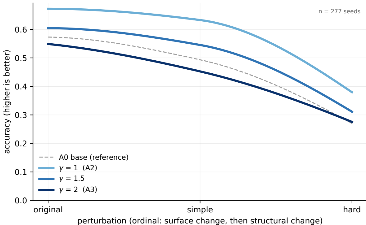
Accuracy-robustness trade-off along \gamma = 1, 1.5, 2 (monotone cubic interpolation through the three arms)
