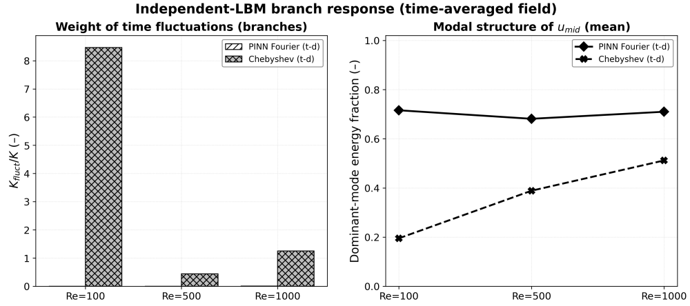
Figure 14: Global temporal response of the LBM realizations under all tested lid controls at Re = 100, 500 , and 1000 . The time-dependent Fourier branch (PINN t -dependent) is quasi-stationary, while the modified-Chebyshev branch remains strongly time-dependent.
