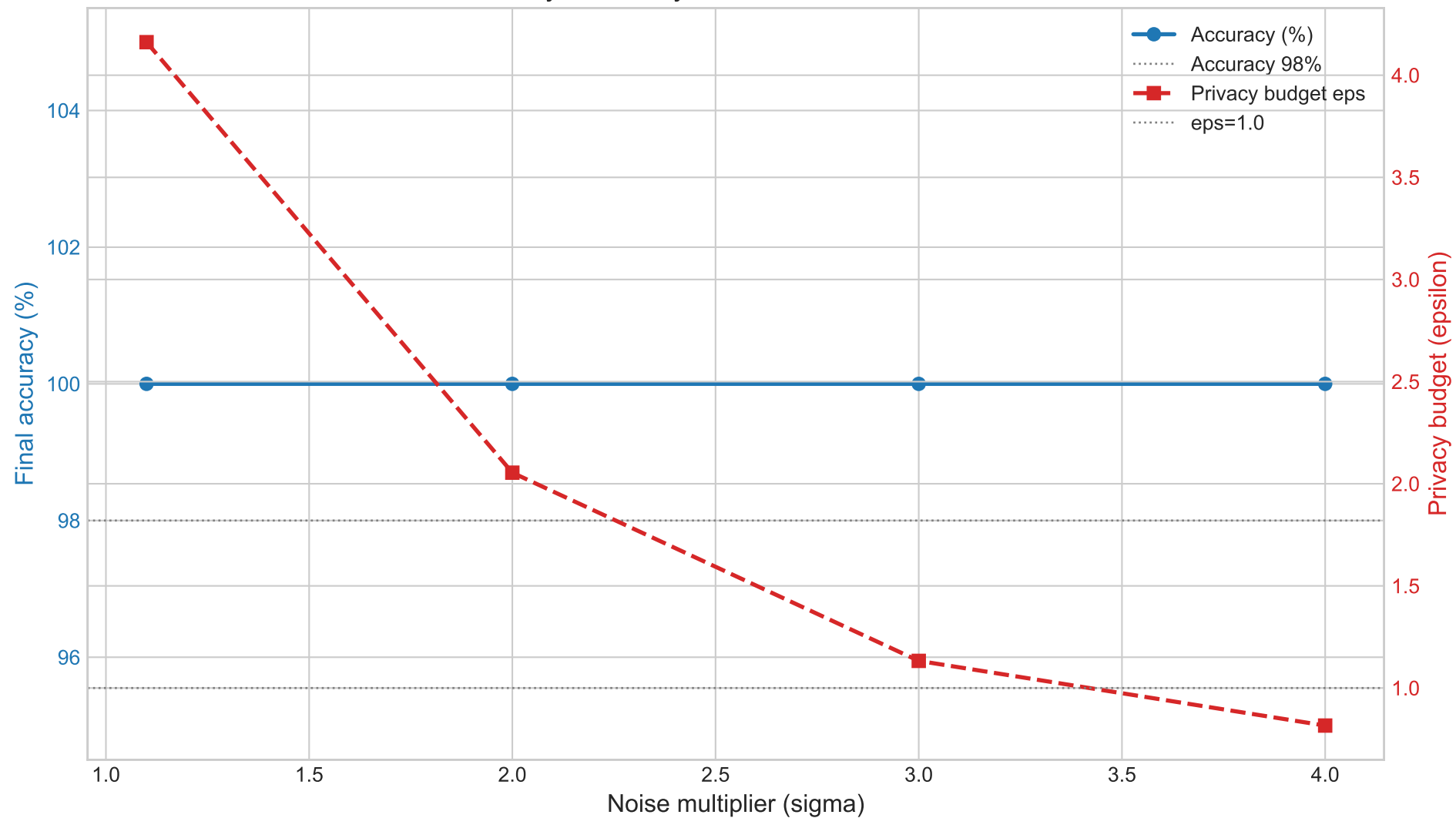
Privacy-Accuracy Tradeoff in PrivFed-TCN
