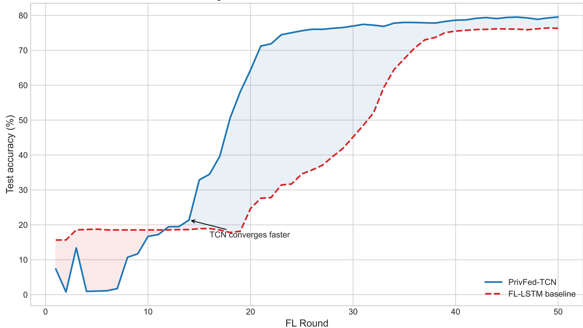
Convergence: PrivFed-TCN vs FL-LSTM Baseline
