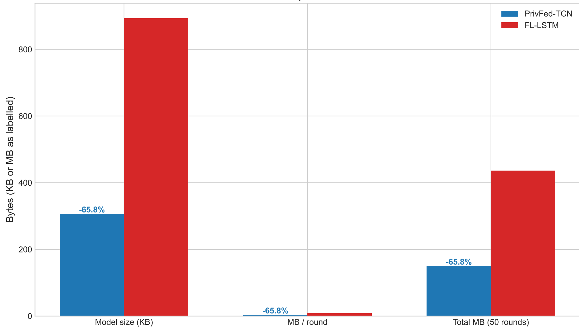
Communication Efficiency: PrivFed-TCN vs FL-LSTM
