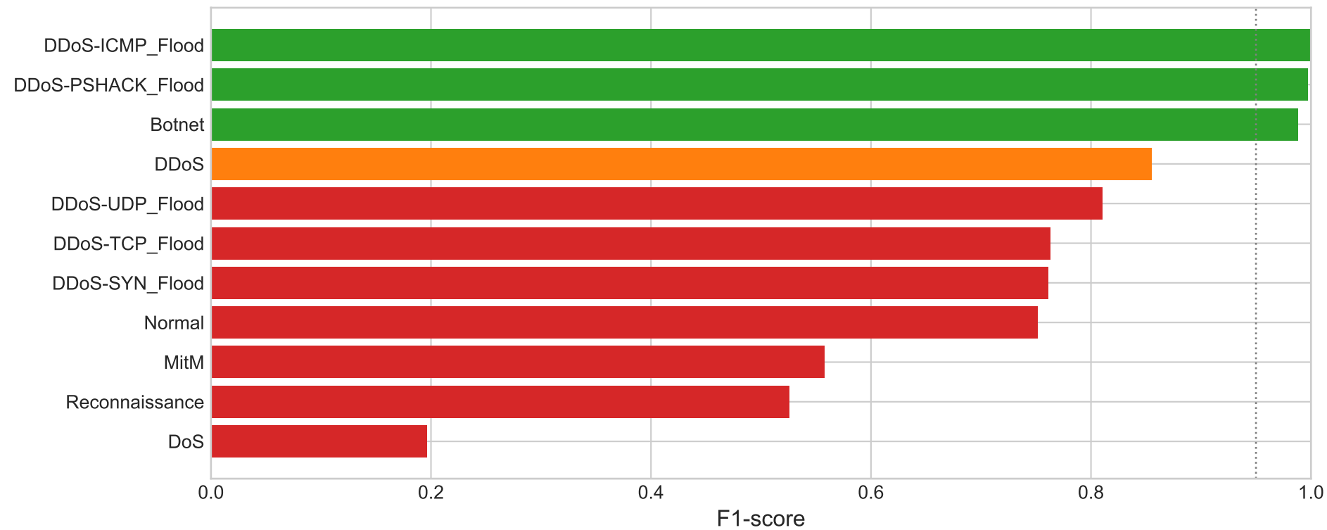
Per-Class F1-Score - PrivFed-TCN
