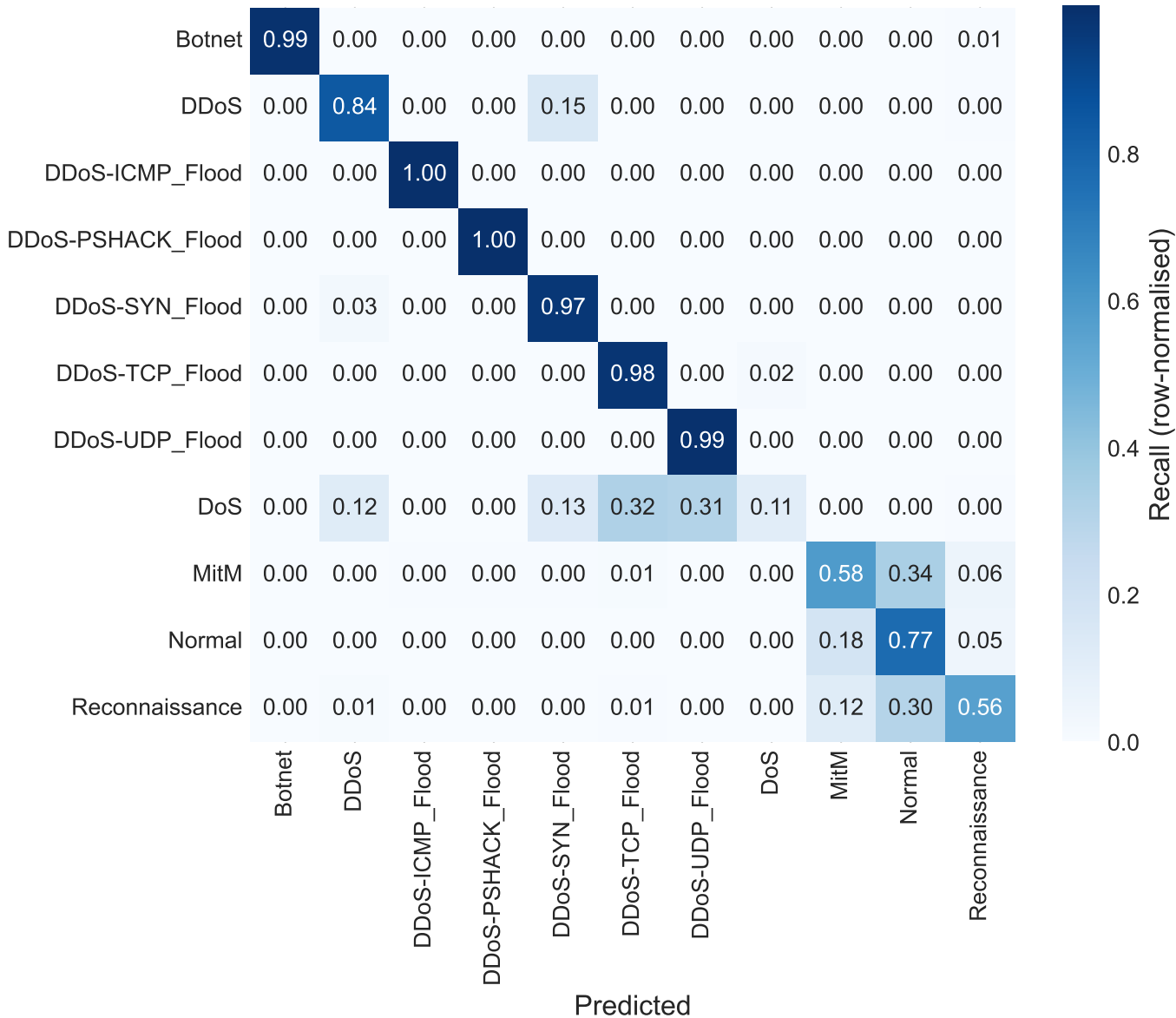
Normalized Confusion Matrix - PrivFed-TCN
