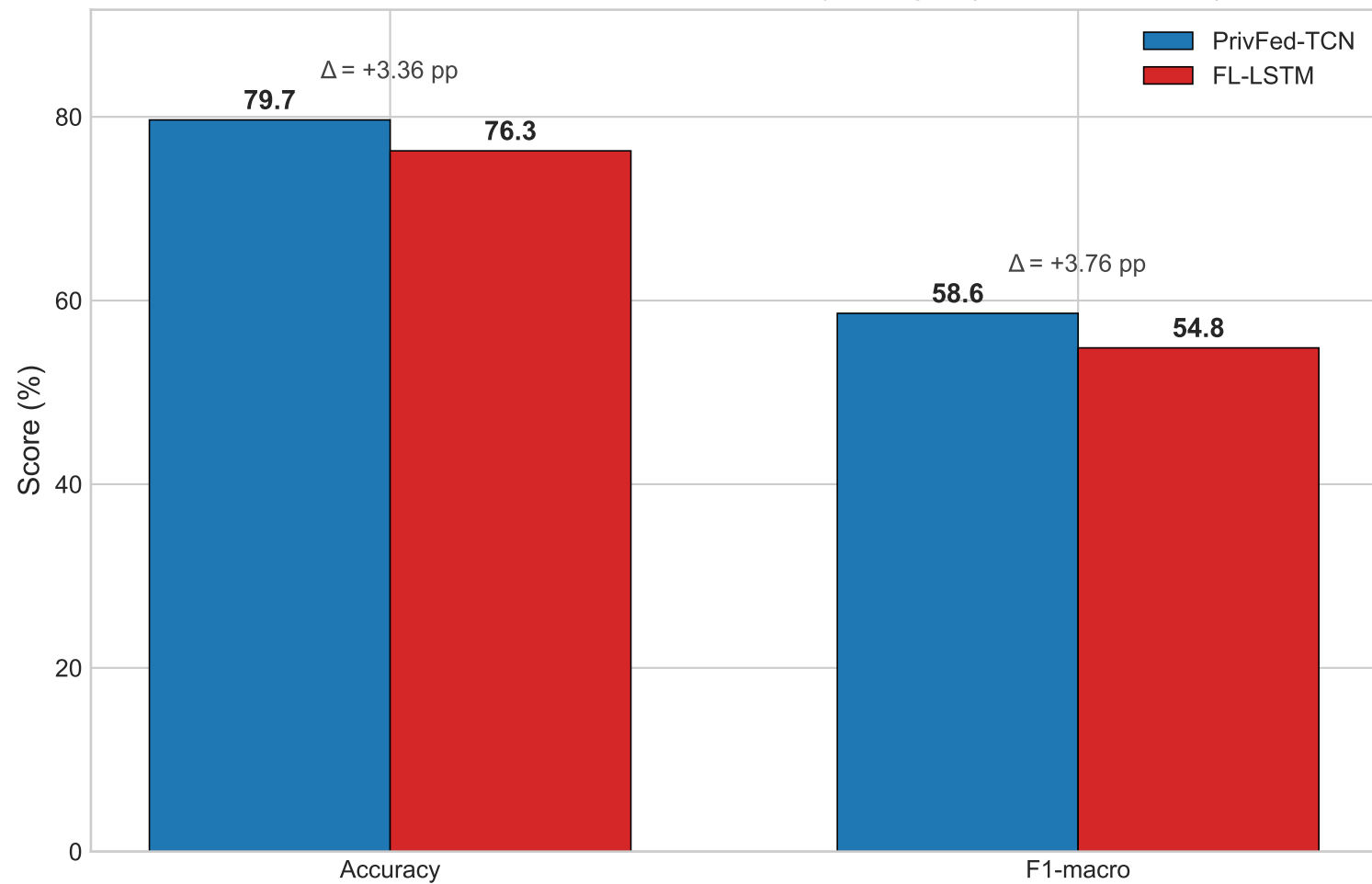
Final Performance under Equal Privacy Budget ( \sigma=10.0 , \epsilon \leq 1.0 )
